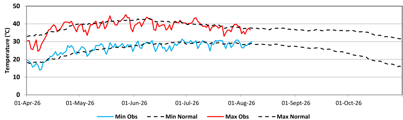
Multan (Min & Max Temperatures)
