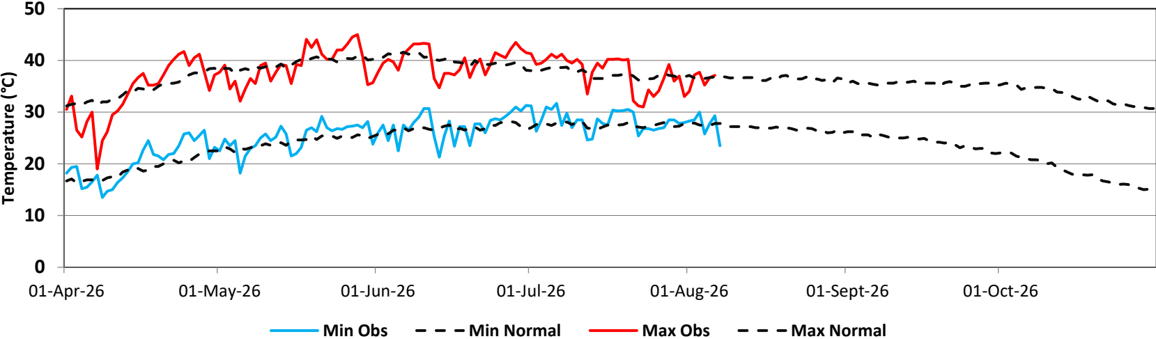
Faisalabad (Min & Max Temperatures)
