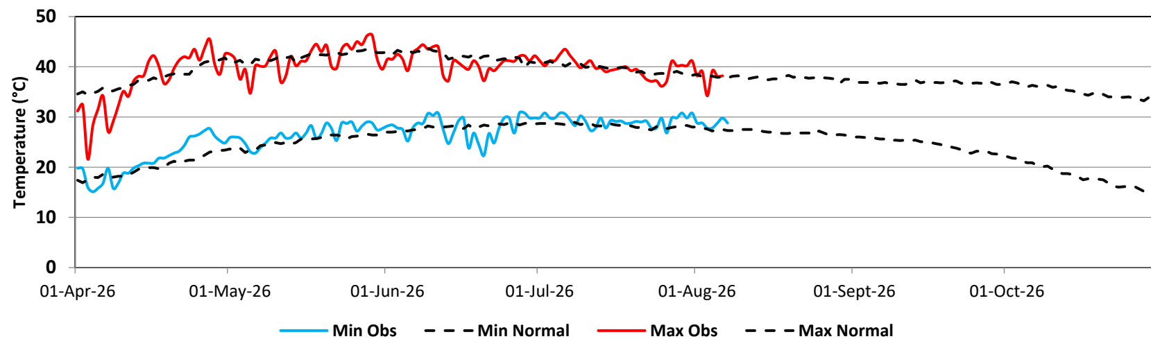
Khanpur (Min & Max Temperatures)
