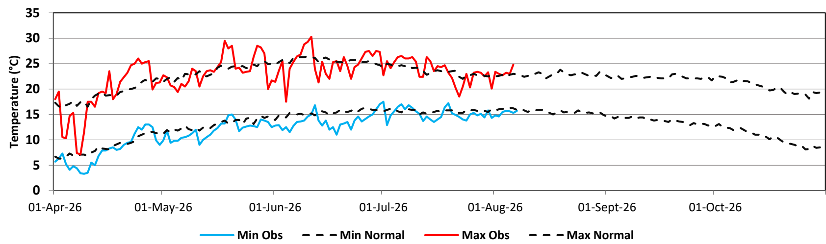
Murree (Min & Max Temperatures)
