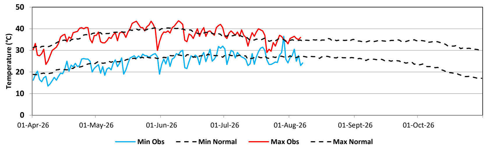
Lahore (Min & Max Temperatures)
