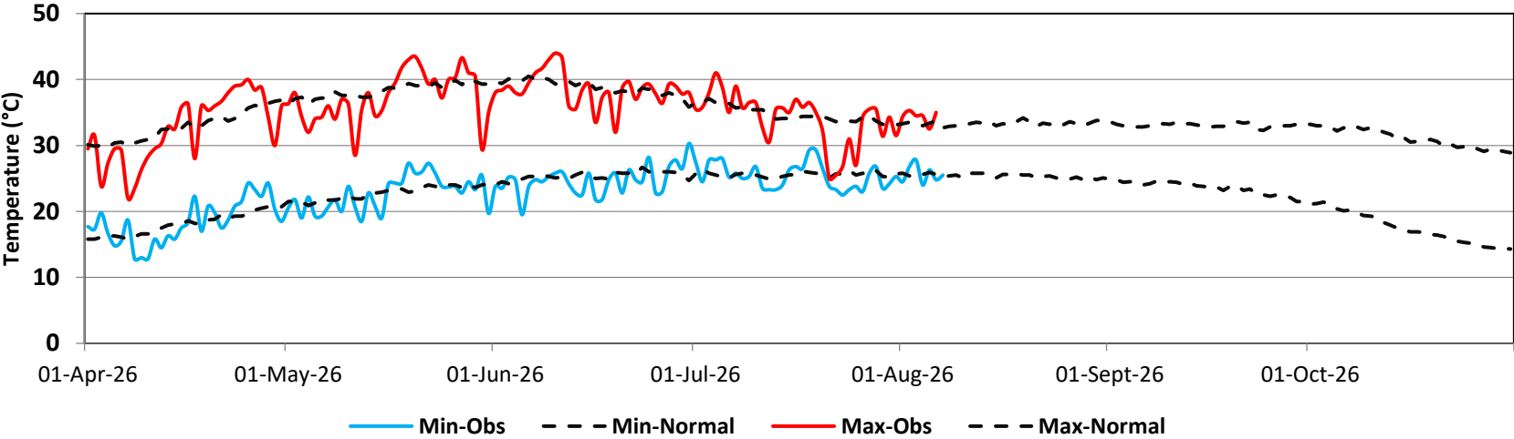
Sialkot (Min & Max Temperatures)
